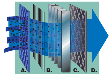
A. Pre-filter screen B. Charging section C. Collecting section D. Charcoal filter (optional)
